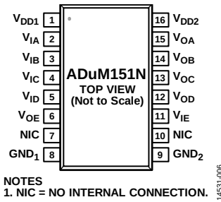
Figure 6. ADuM151N Pin Configuration
