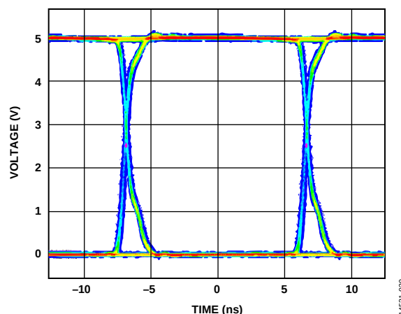
Figure 20. ADuM150N/ADuM151N/ADuM152N Eye Diagram
